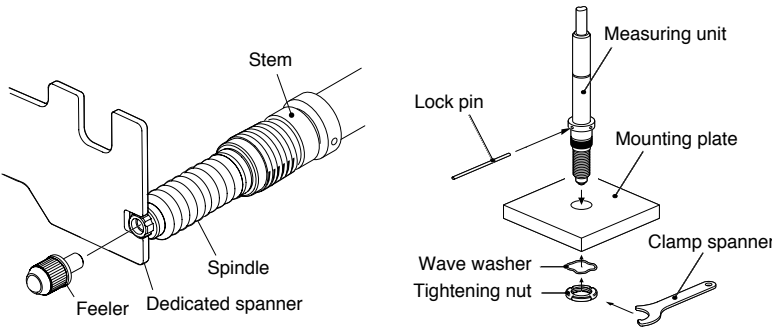
Feeler installation/removal method
