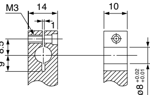
Moutint holder dimension
