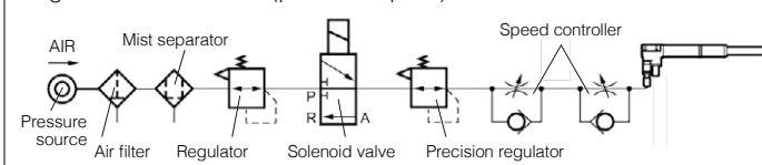
Fig. 1 Pneumatic circuit (pneumatic push)
