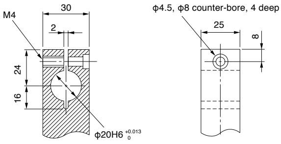
Mounting holder dimenstions and tolerance
