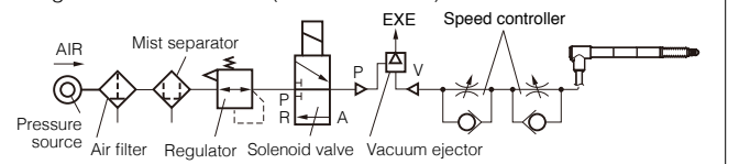
Fig. 2 Pneumatic circuit (vacuum suction)
