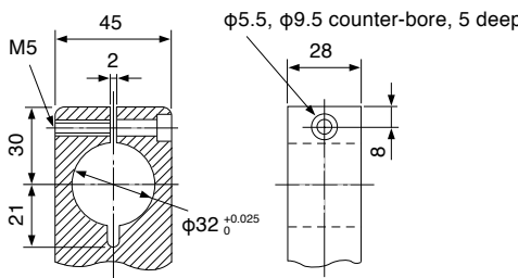
Mouting holder dimenstions and tolerance
