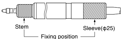
Mounting/fixing position
