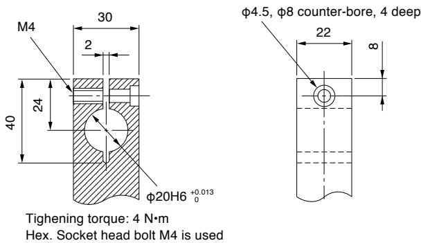
Mounting holder dimenstions and tolerance
