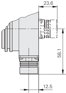
M23 flange socket
